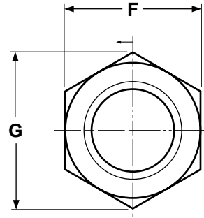
Nylon Insert Stop Nuts, Thin Pattern
