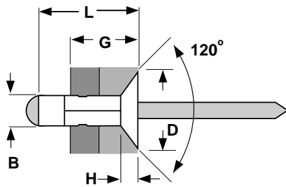
COUNTERSUNK HEAD
