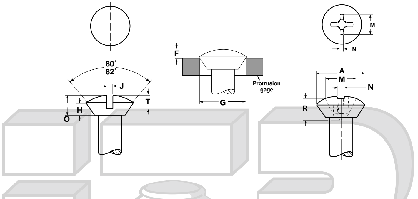
UNDERCUT OVAL HEADS FOR MACHINE SCREWS
