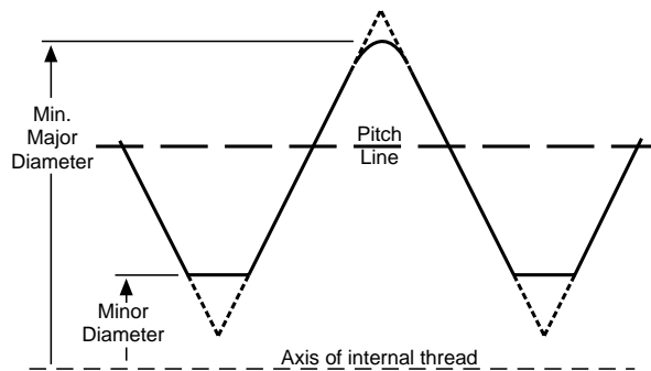
INTERNAL THREADS - CLASS 2B (CONTINUED)
